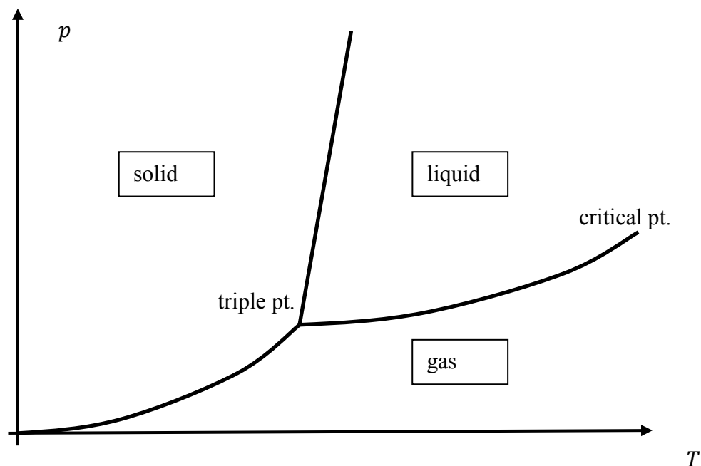
Fig. 2.16: p-T-phase diagram
